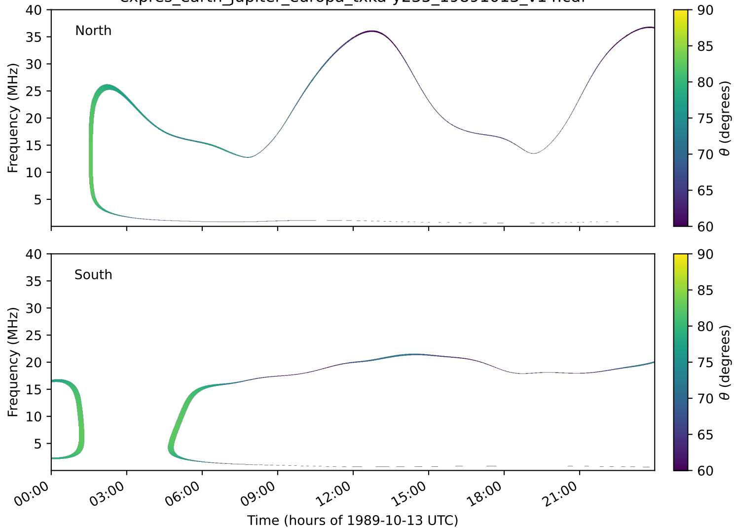
expres_earth_jupiter_europa_txka-y235_19891013_v14.cdf
