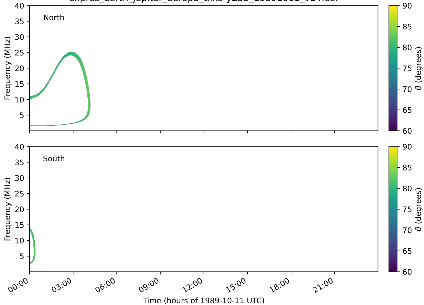
expres_earth_jupiter_europa_txka-y235_19891011_v14.cdf
