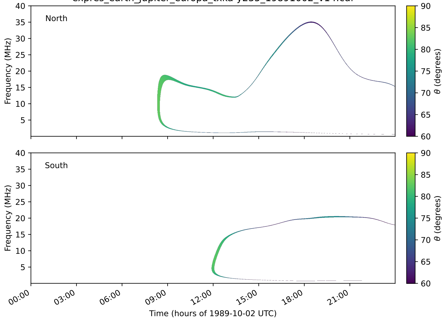
expres_earth_jupiter_europa_txka-y235_19891002_v14.cdf
