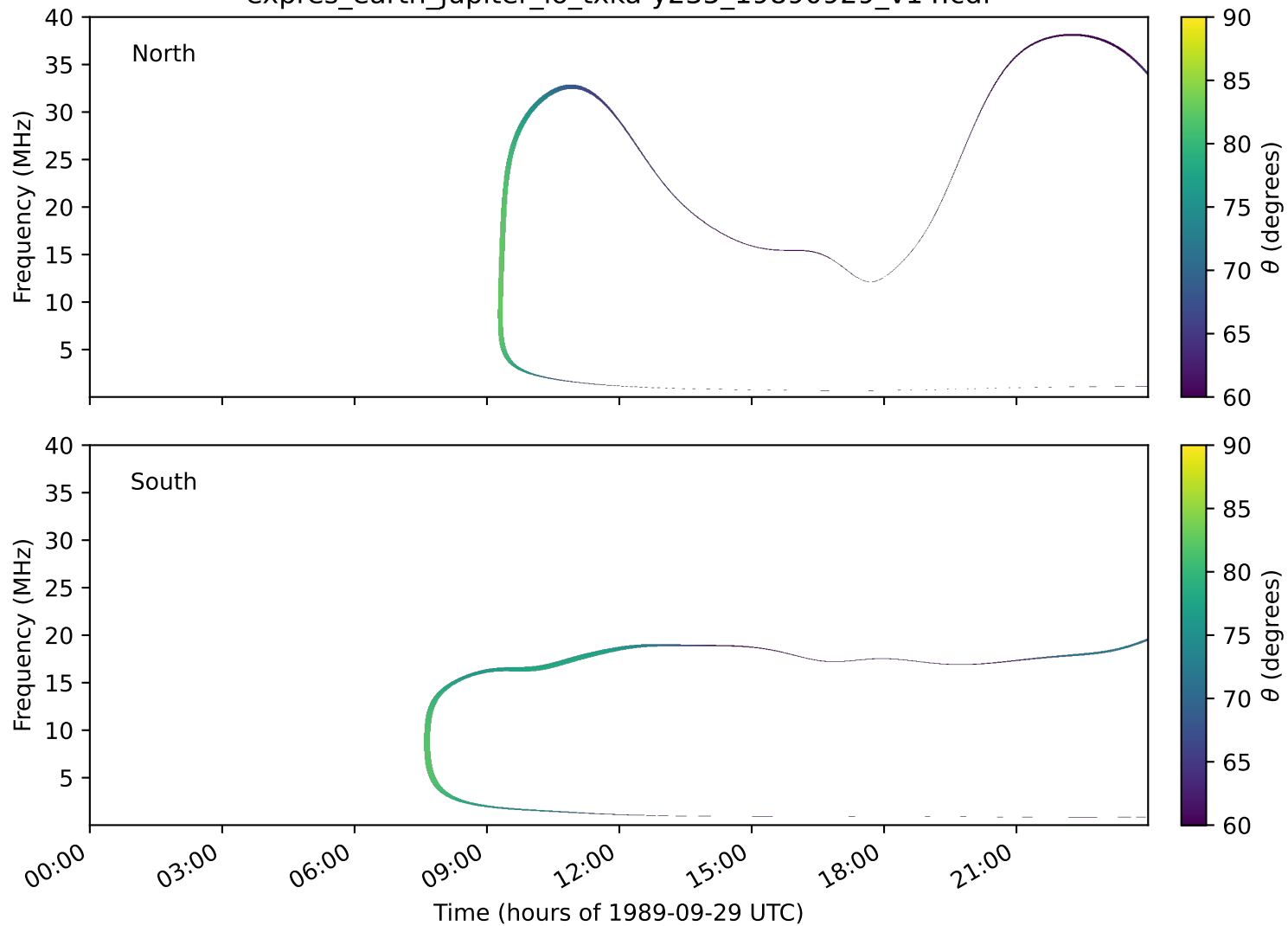
expres_earth_jupiter_io_txka-y235_19890929_v14.cdf
