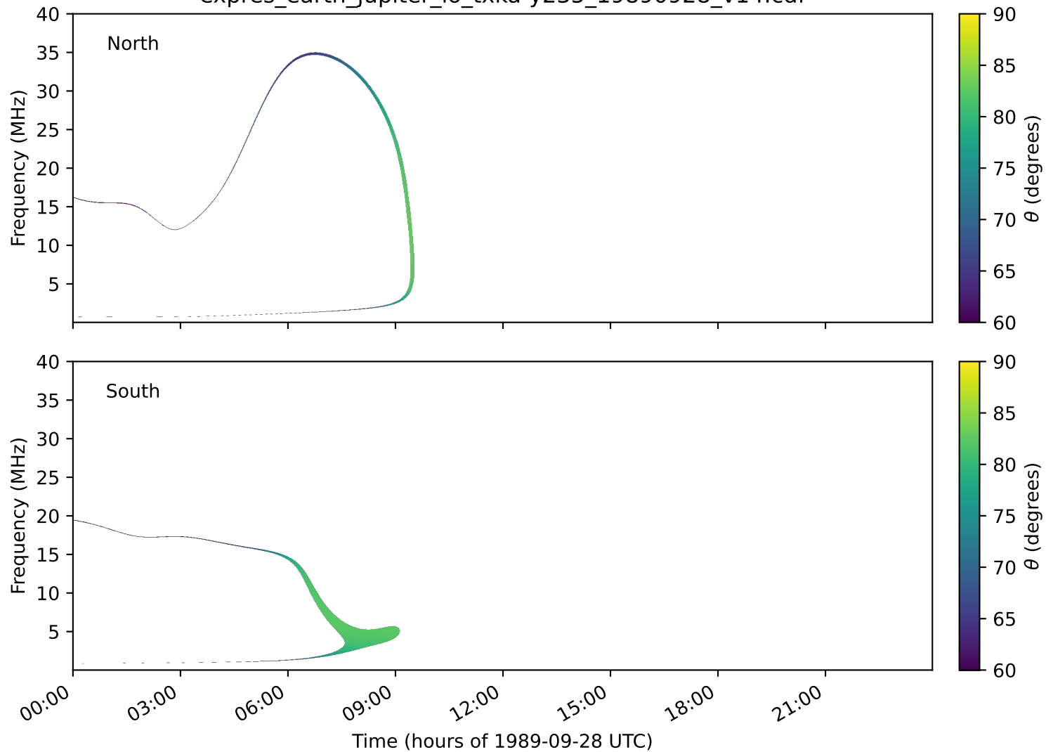
expres_earth_jupiter_io_txka-y235_19890928_v14.cdf
