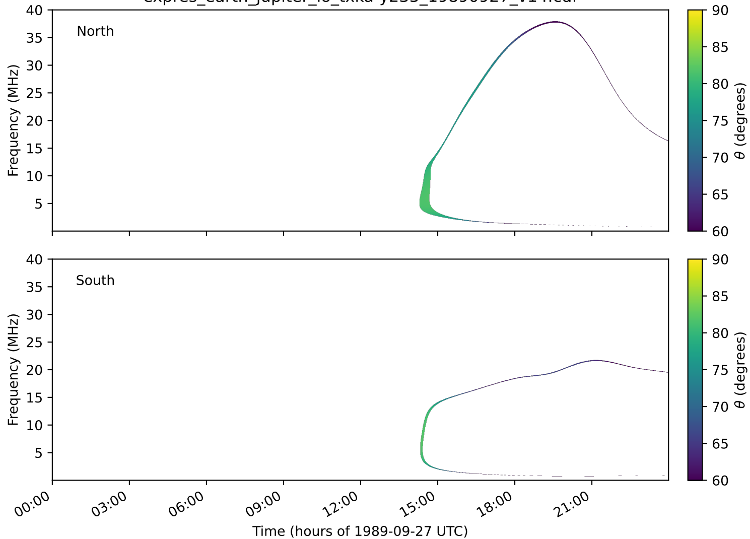
expres_earth_jupiter_io_txka-y235_19890927_v14.cdf
