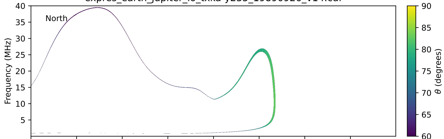
expres_earth_jupiter_io_txka-y235_19890926_v14.cdf
