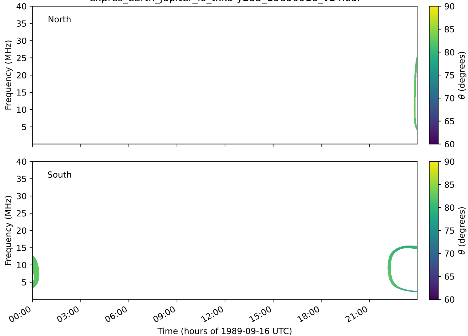
expres_earth_jupiter_io_txka-y235_19890916_v14.cdf
