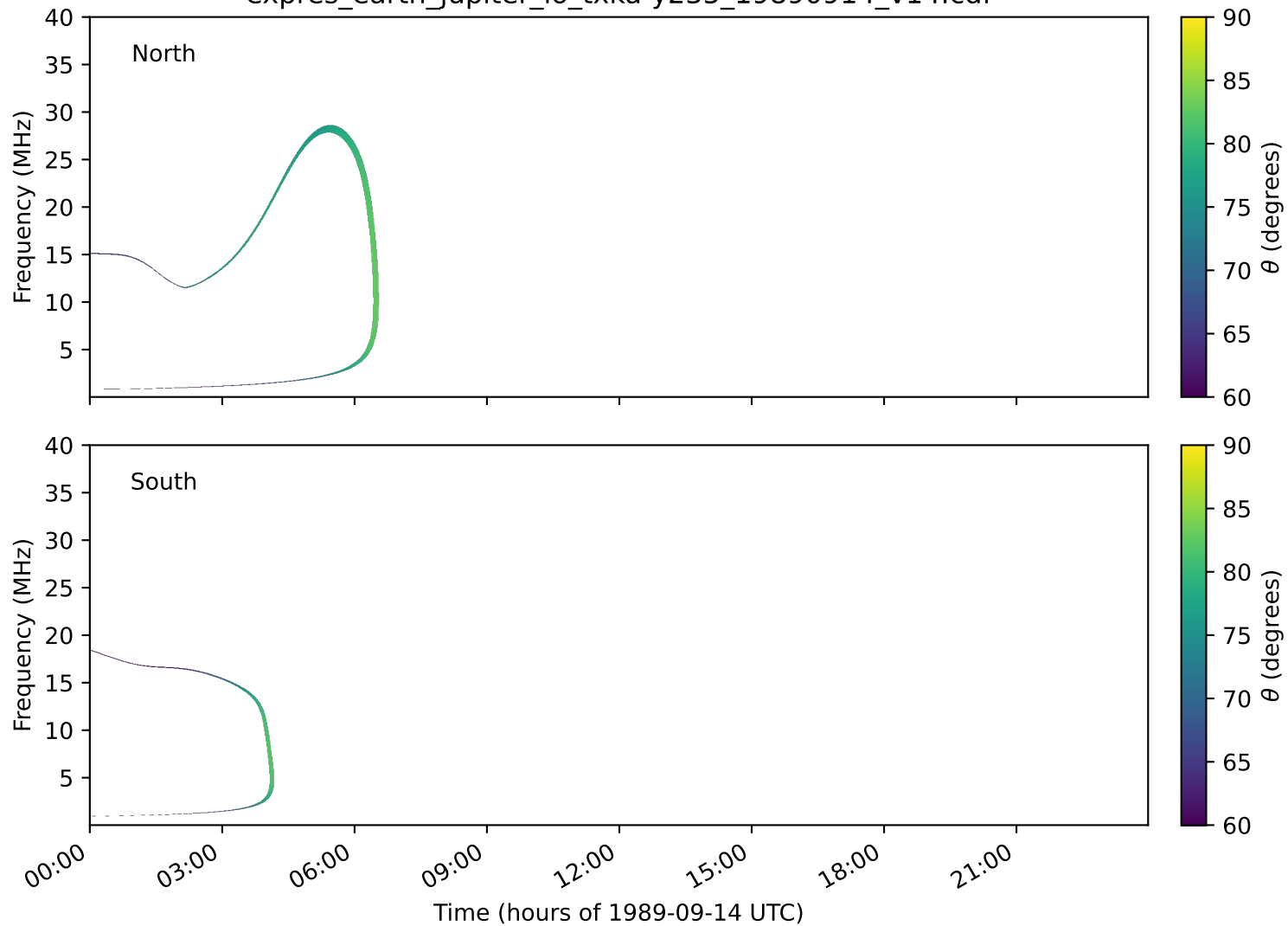
expres_earth_jupiter_io_txka-y235_19890914_v14.cdf
