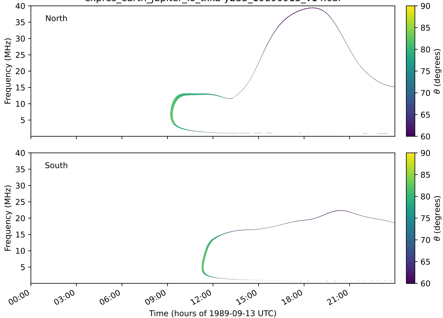
expres_earth_jupiter_io_txka-y235_19890913_v14.cdf
