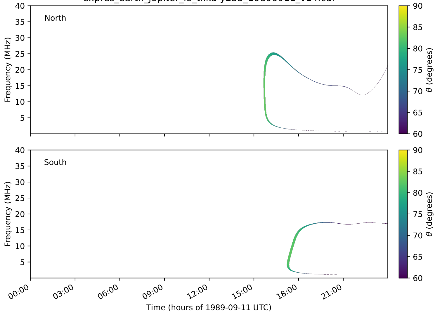
expres_earth_jupiter_io_txka-y235_19890911_v14.cdf
