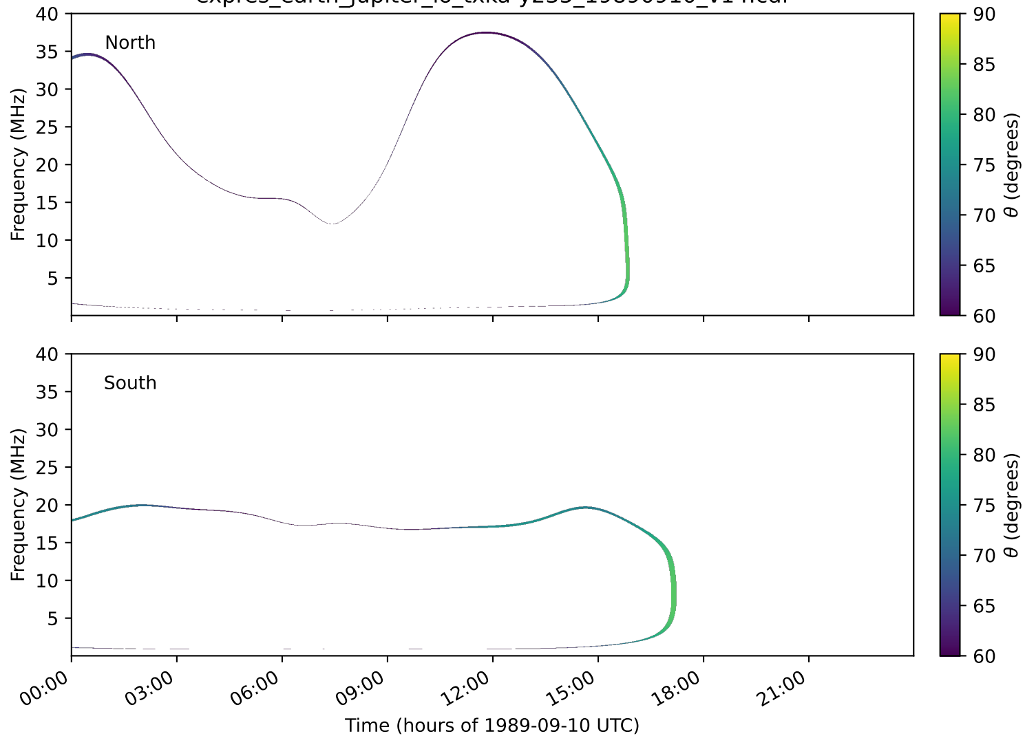
expres_earth_jupiter_io_txka-y235_19890910_v14.cdf
