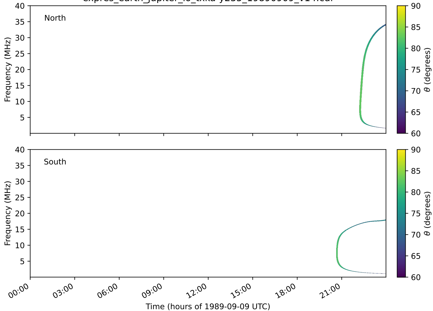
expres_earth_jupiter_io_txka-y235_19890909_v14.cdf
