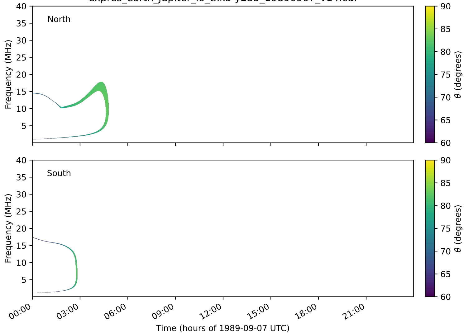
expres_earth_jupiter_io_txka-y235_19890907_v14.cdf
