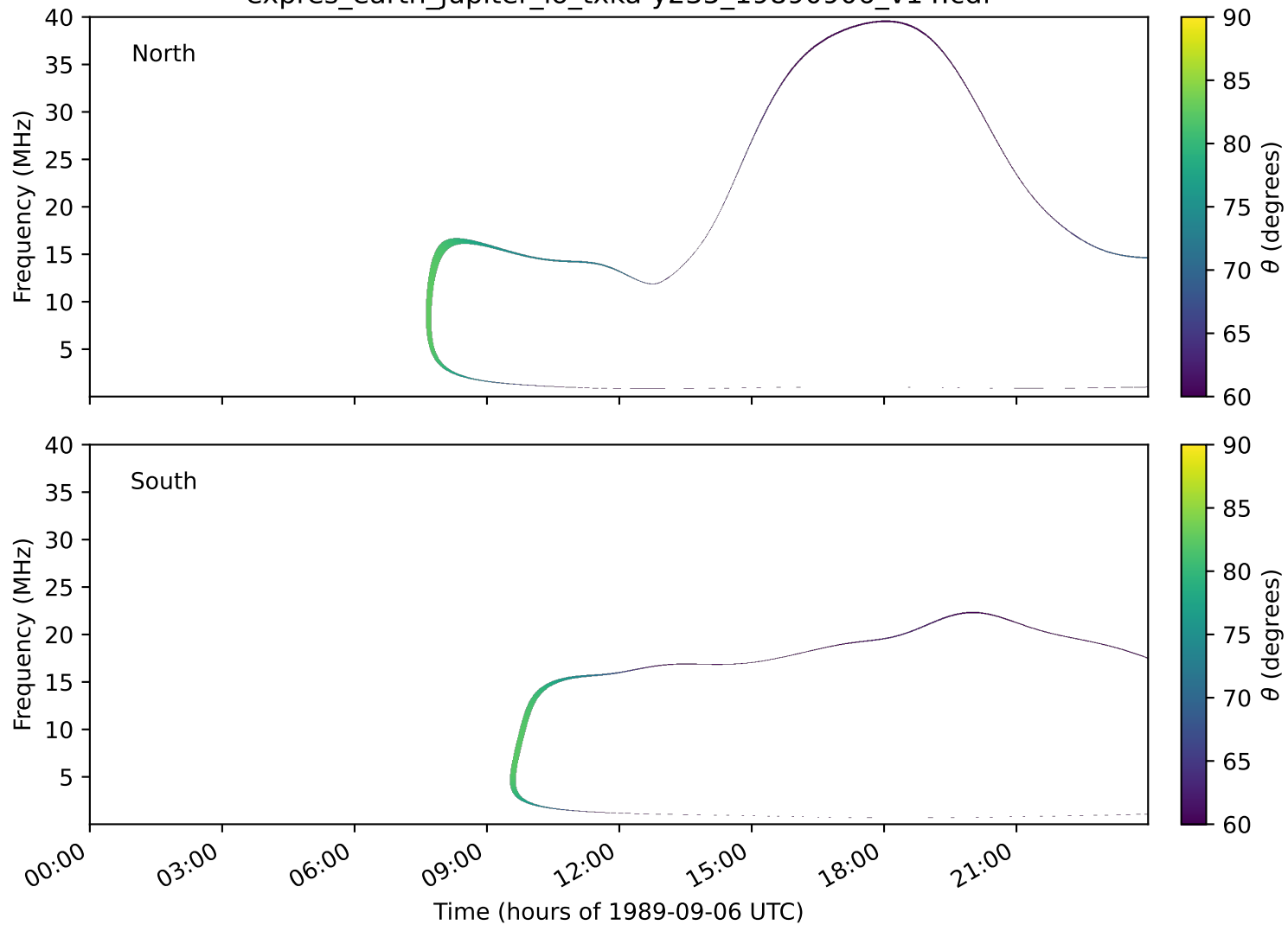
expres_earth_jupiter_io_txka-y235_19890906_v14.cdf
