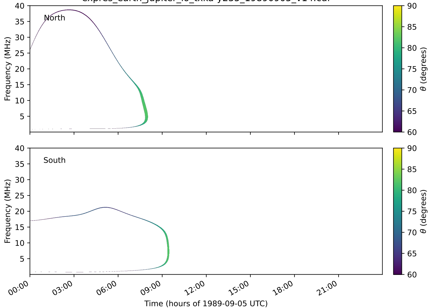
expres_earth_jupiter_io_txka-y235_19890905_v14.cdf
