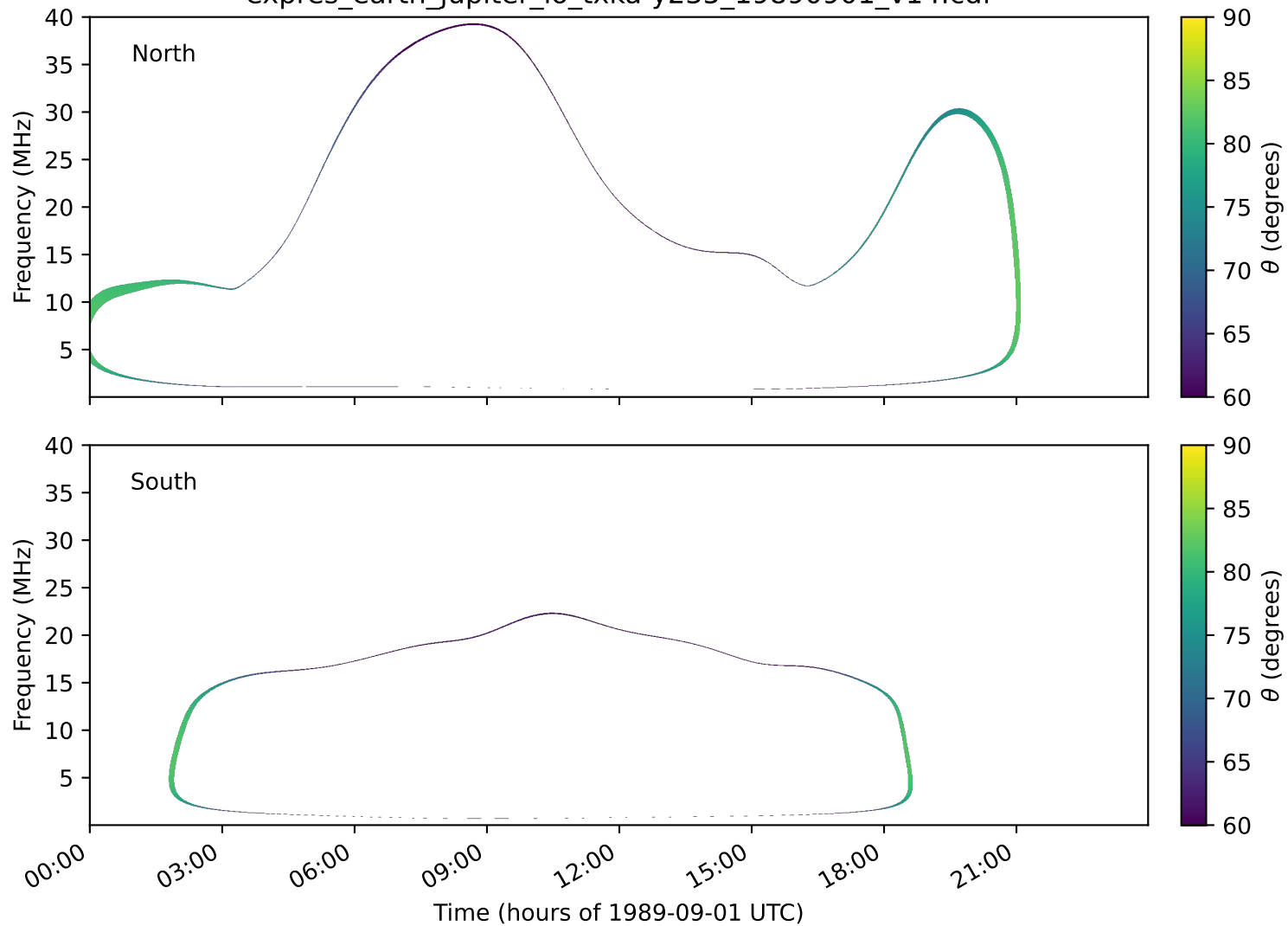
expres_earth_jupiter_io_txka-y235_19890901_v14.cdf
