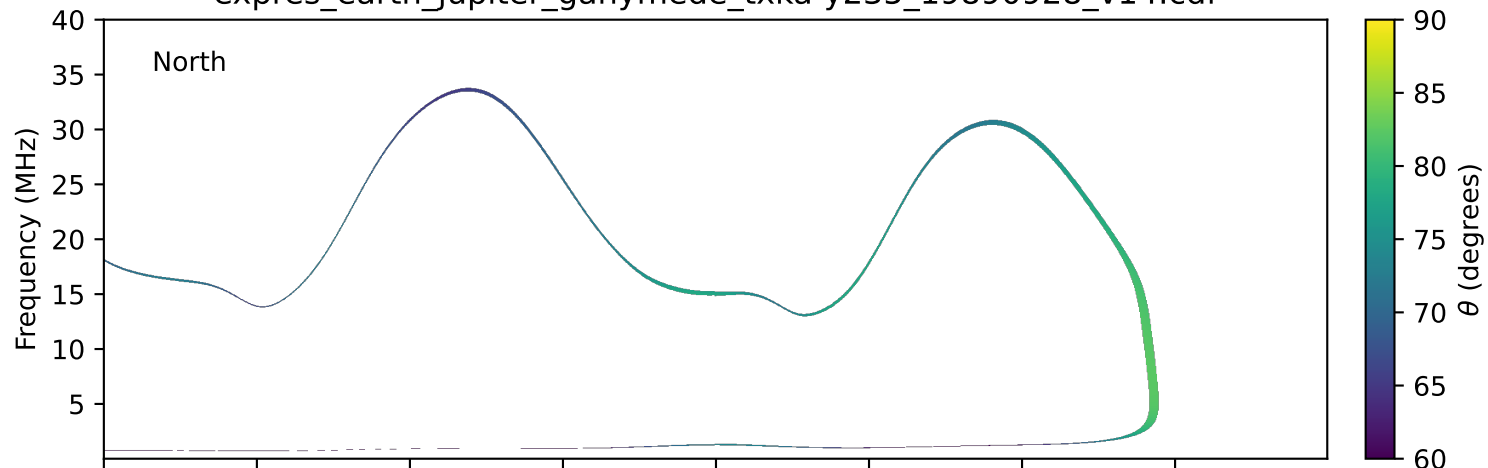
expres_earth_jupiter_ganymede_txka-y235_19890928_v14.cdf
