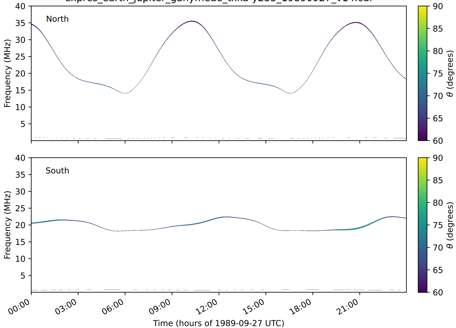
expres_earth_jupiter_ganymede_txka-y235_19890927_v14.cdf
