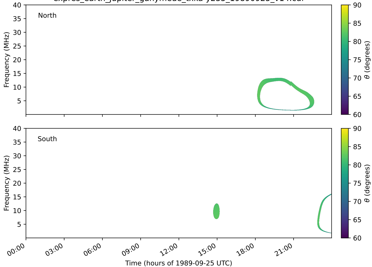
expres_earth_jupiter_ganymede_txka-y235_19890925_v14.cdf
