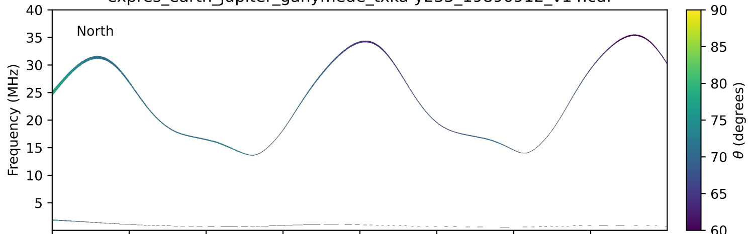
expres_earth_jupiter_ganymede_txka-y235_19890912_v14.cdf
