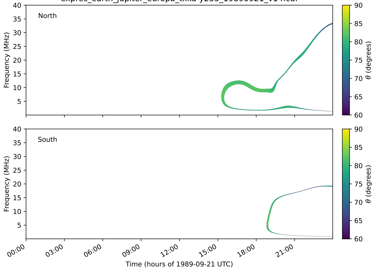
expres_earth_jupiter_europa_txka-y235_19890921_v14.cdf
