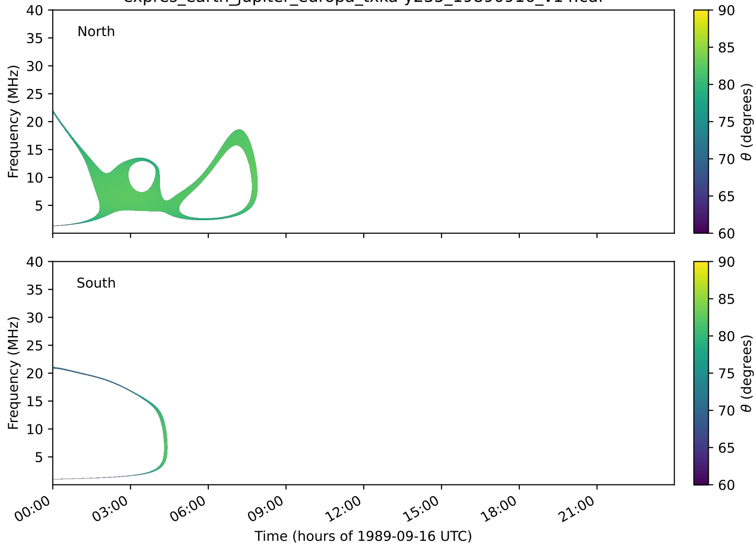
expres_earth_jupiter_europa_txka-y235_19890916_v14.cdf
