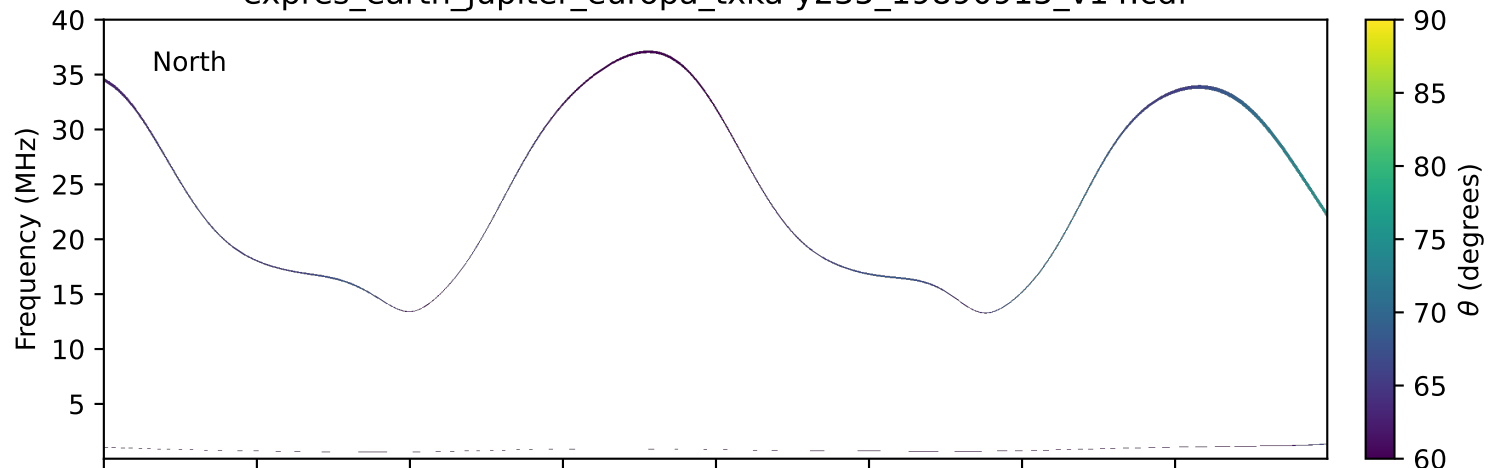
expres_earth_jupiter_europa_txka-y235_19890915_v14.cdf
