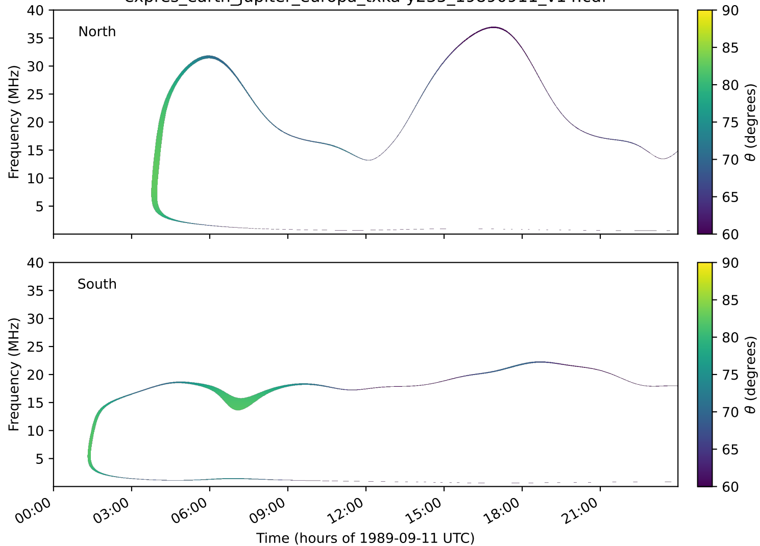
expres_earth_jupiter_europa_txka-y235_19890911_v14.cdf
