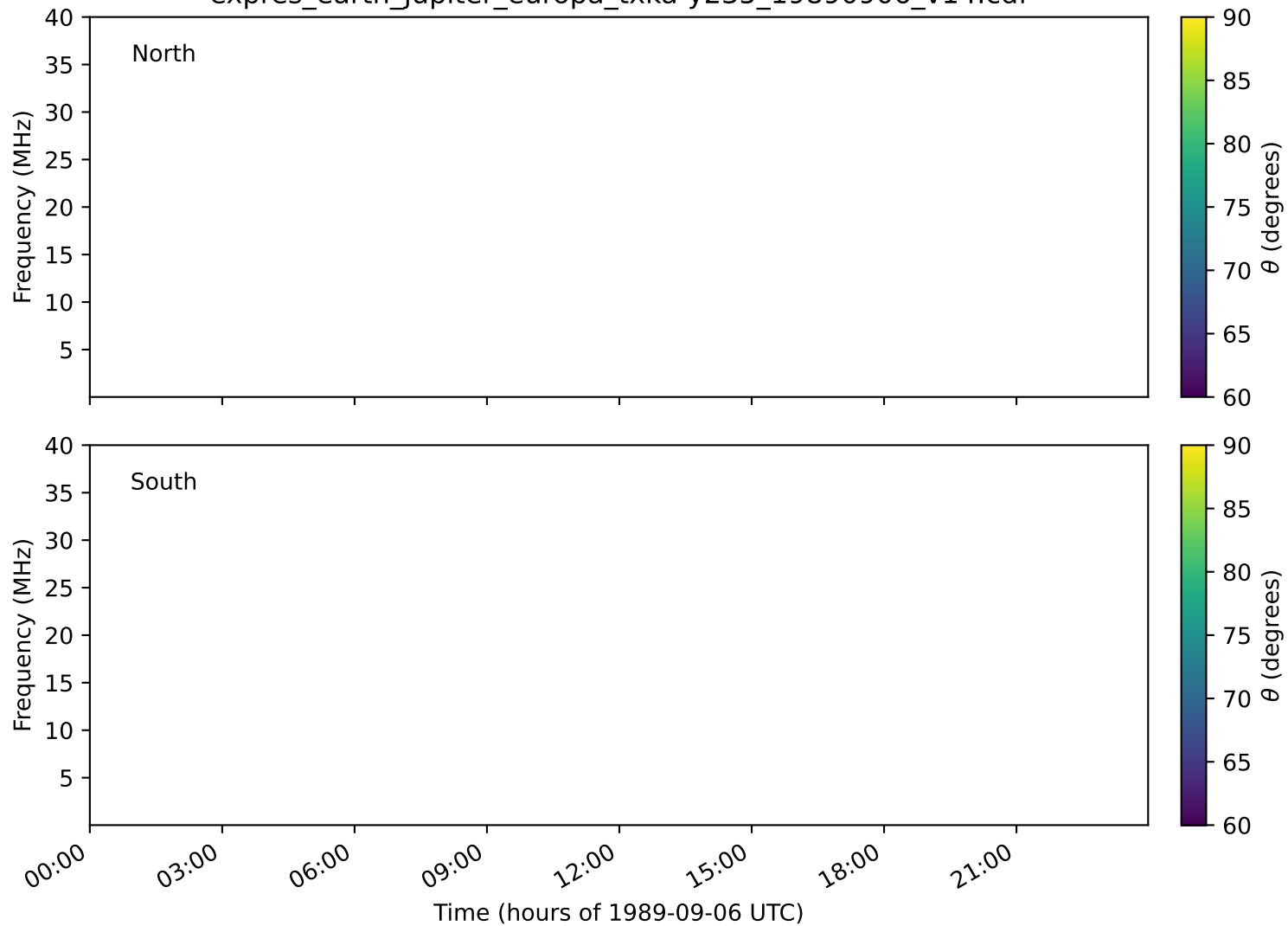
expres_earth_jupiter_europa_txka-y235_19890906_v14.cdf
