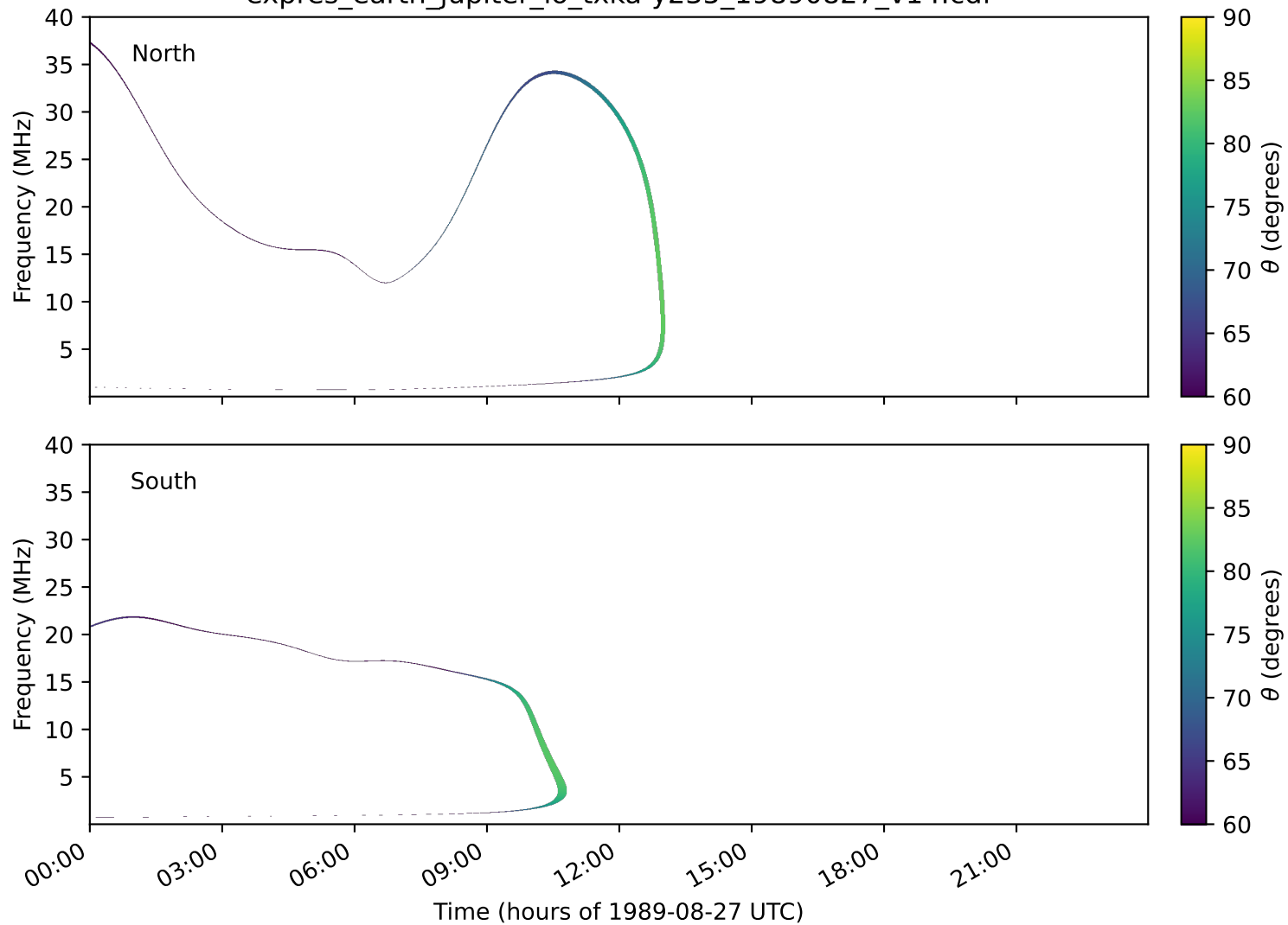
expres_earth_jupiter_io_txka-y235_19890827_v14.cdf
