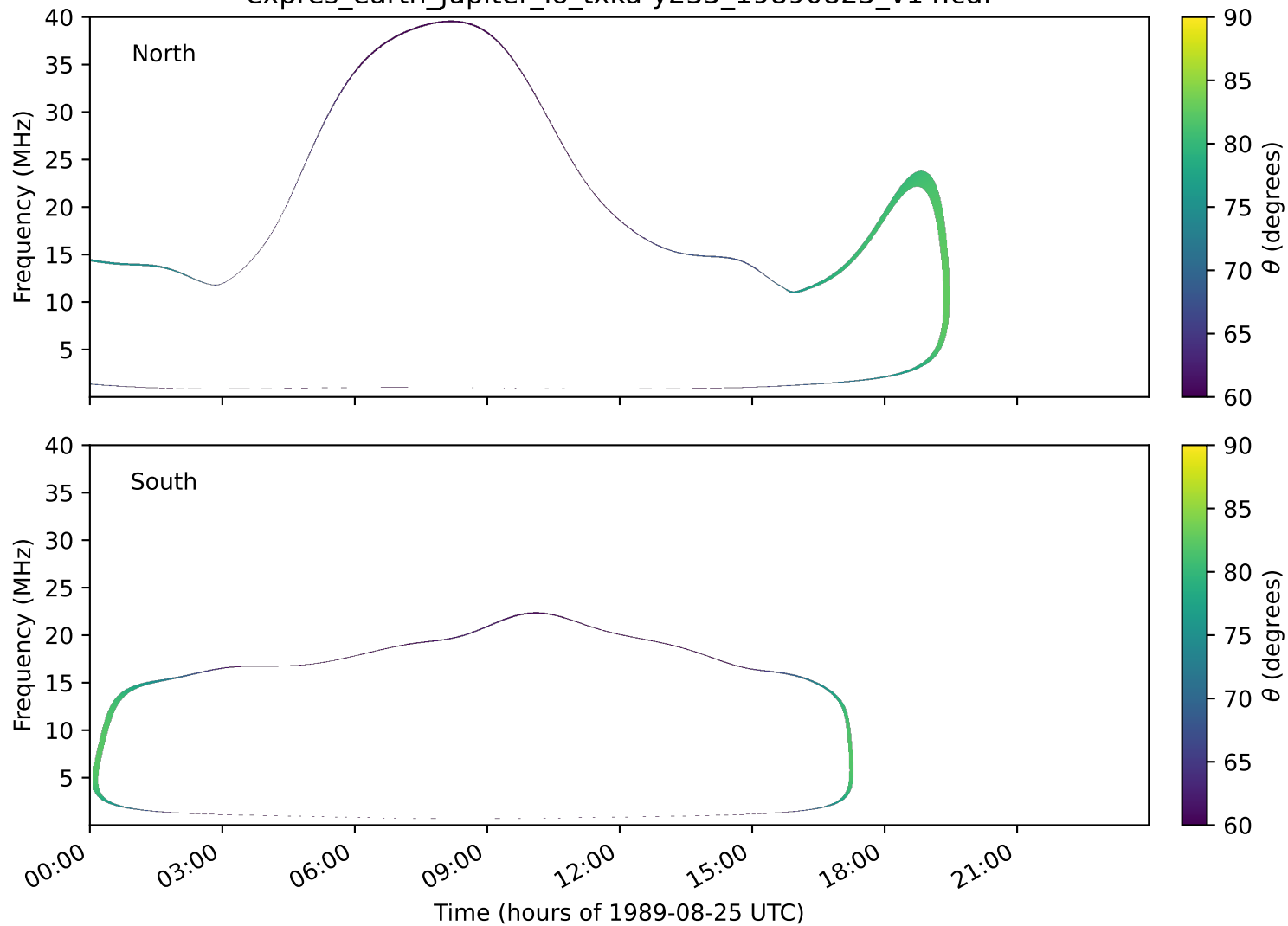
expres_earth_jupiter_io_txka-y235_19890825_v14.cdf
