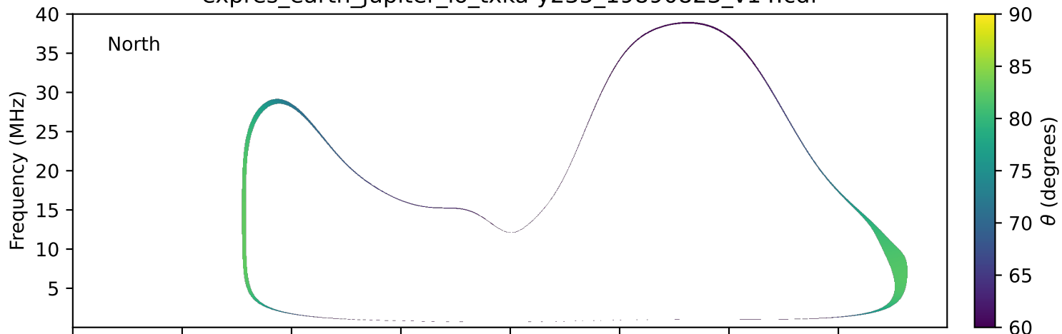
expres_earth_jupiter_io_txka-y235_19890823_v14.cdf
