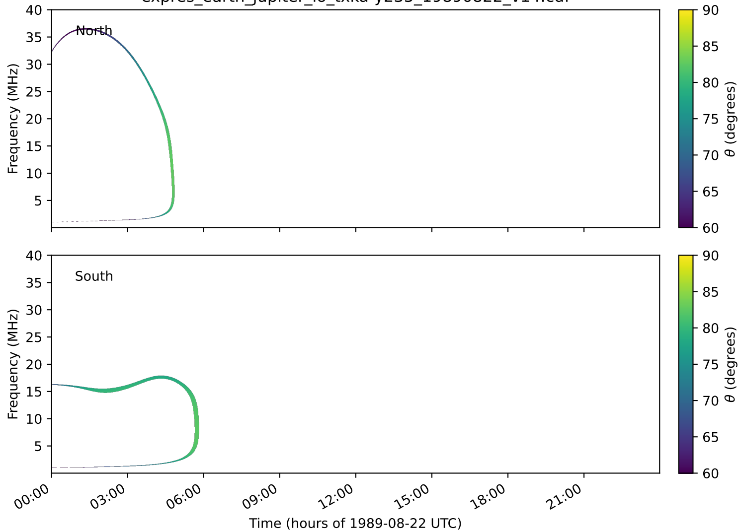
expres_earth_jupiter_io_txka-y235_19890822_v14.cdf
