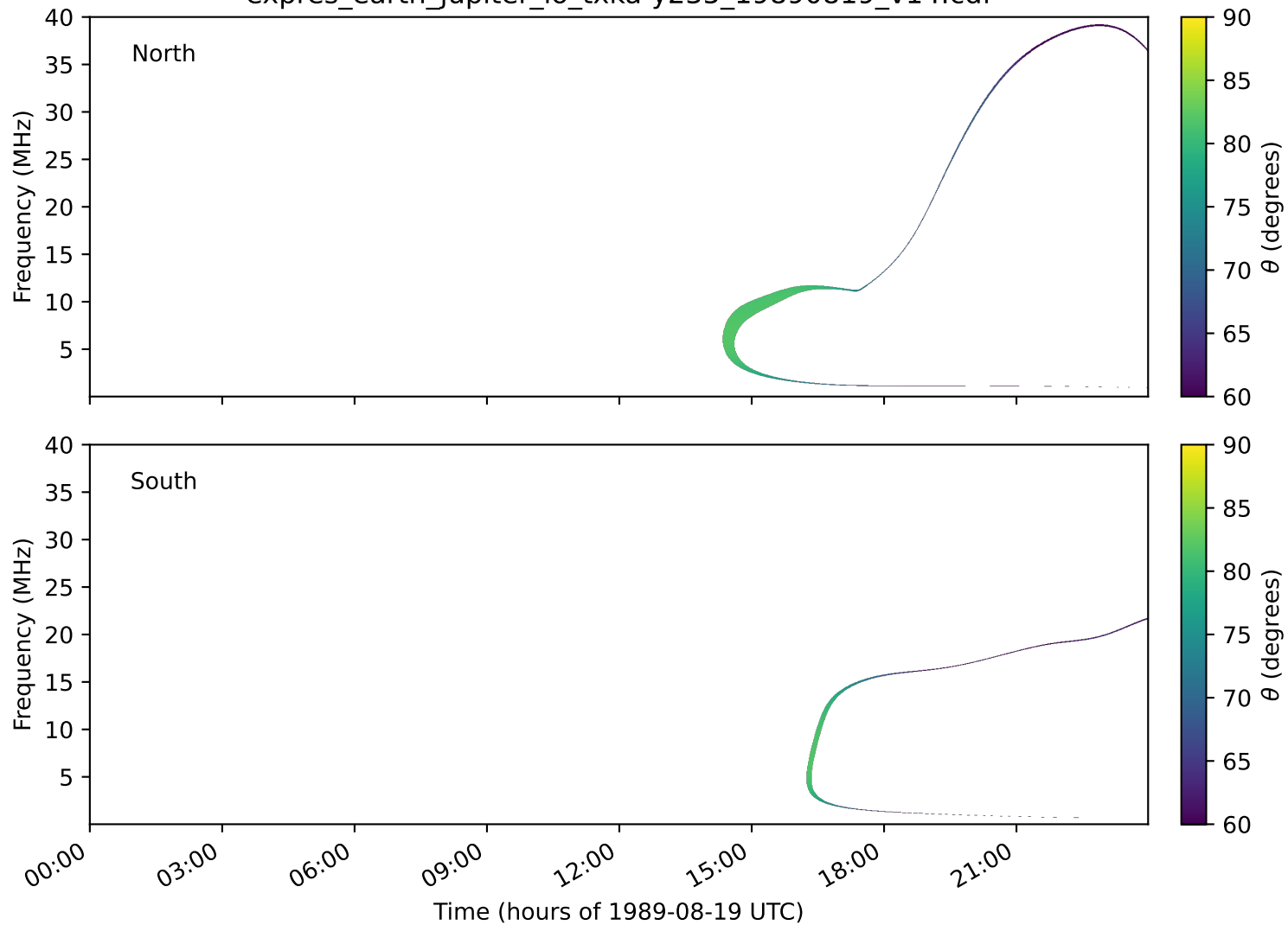
expres_earth_jupiter_io_txka-y235_19890819_v14.cdf
