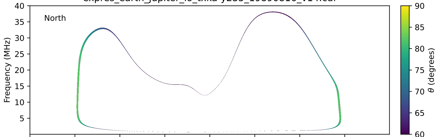
expres_earth_jupiter_io_txka-y235_19890816_v14.cdf
