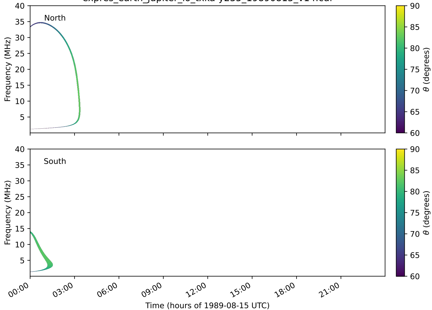
expres_earth_jupiter_io_txka-y235_19890815_v14.cdf
