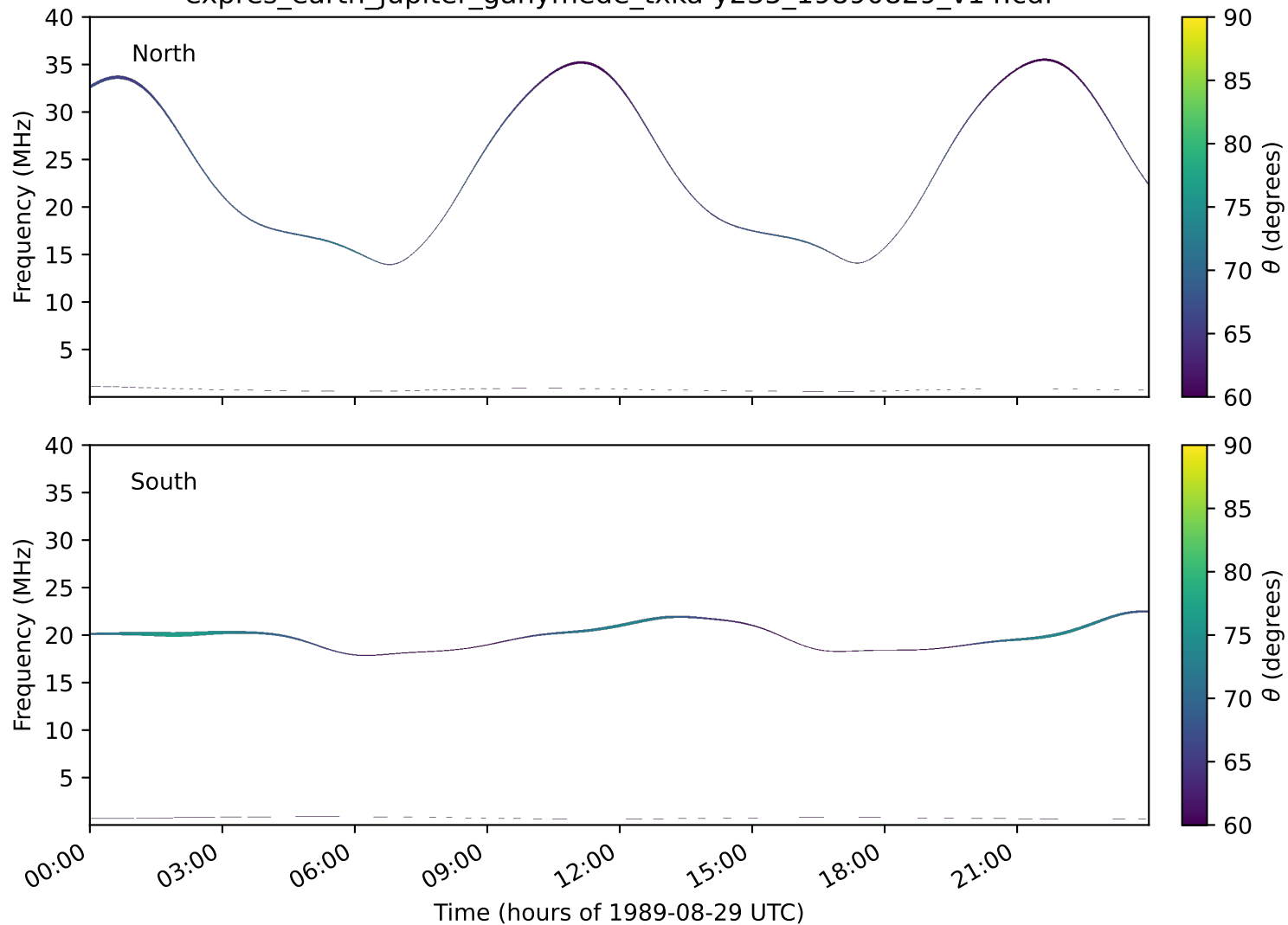
expres_earth_jupiter_ganymede_txka-y235_19890829_v14.cdf
