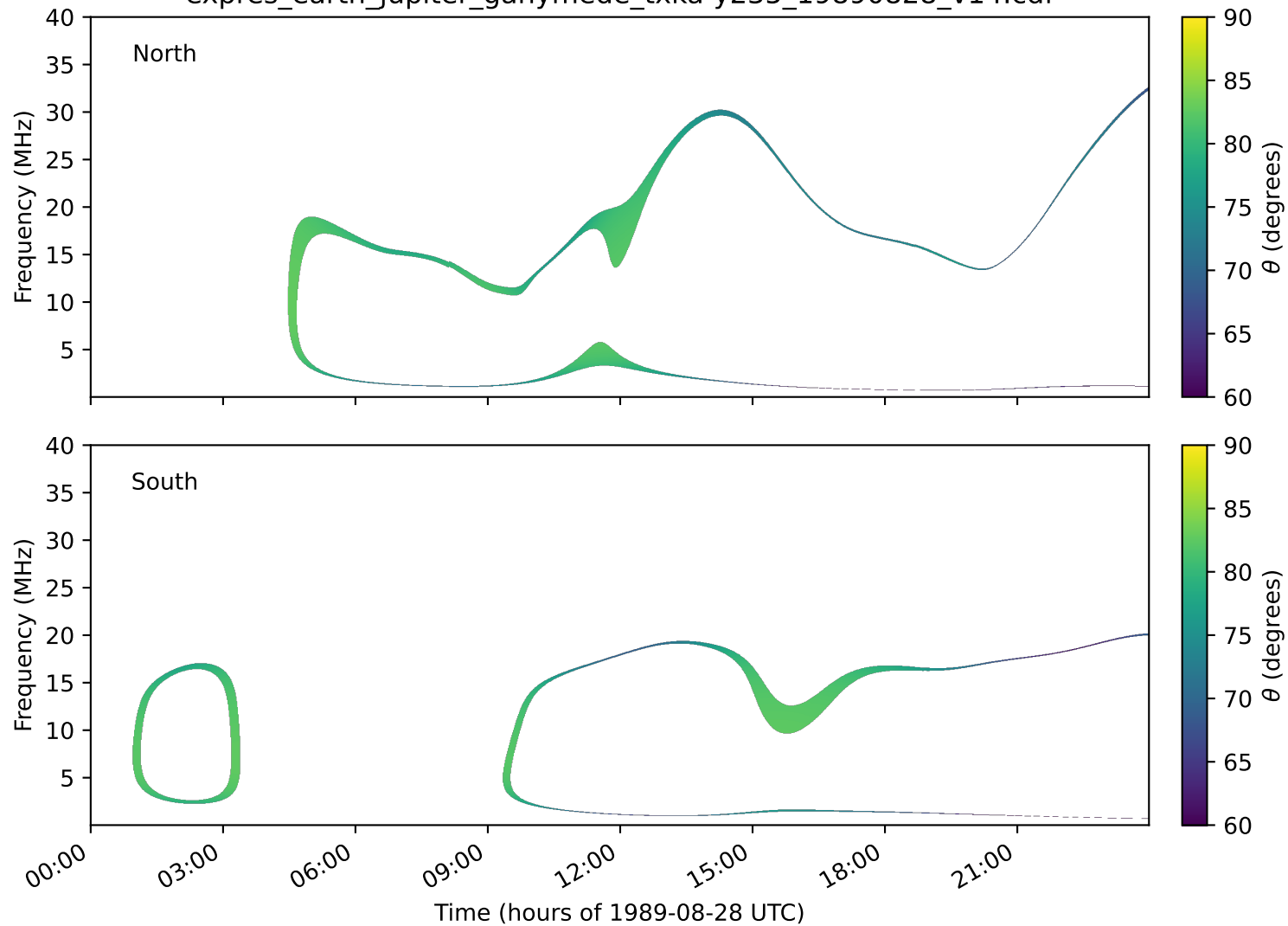
expres_earth_jupiter_ganymede_txka-y235_19890828_v14.cdf
