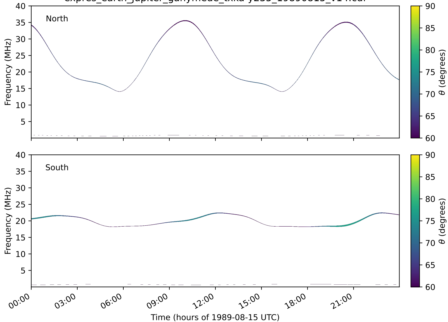
expres_earth_jupiter_ganymede_txka-y235_19890815_v14.cdf
