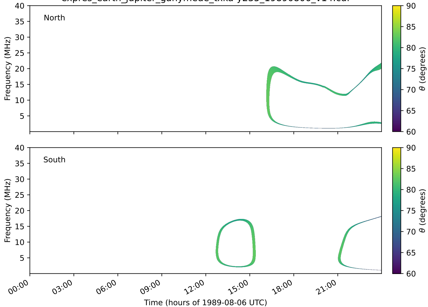
expres_earth_jupiter_ganymede_txka-y235_19890806_v14.cdf
