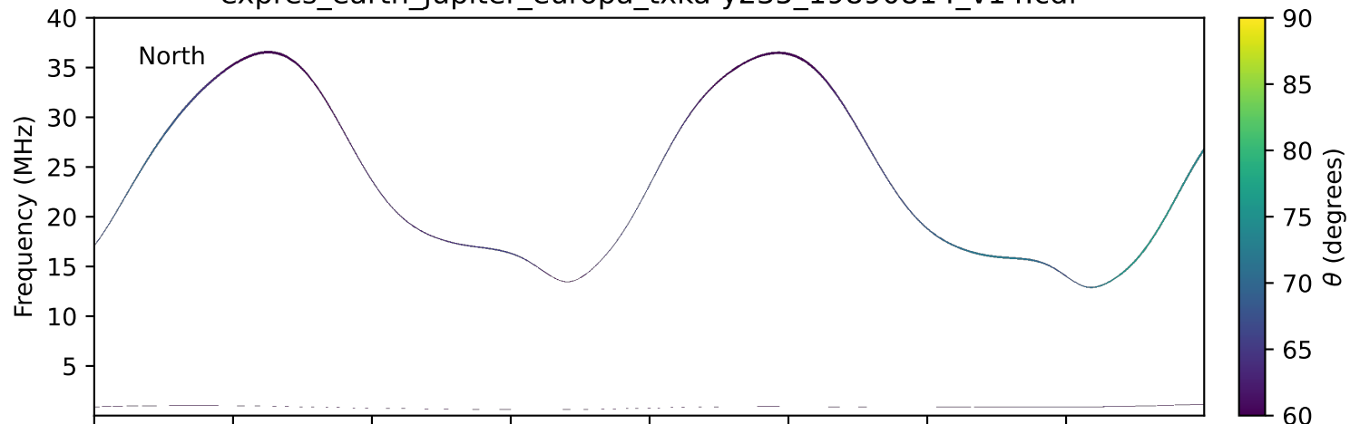
expres_earth_jupiter_europa_txka-y235_19890814_v14.cdf
