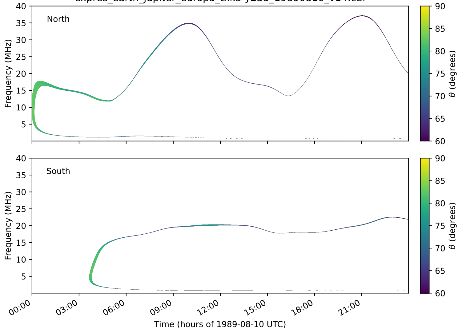
expres_earth_jupiter_europa_txka-y235_19890810_v14.cdf
