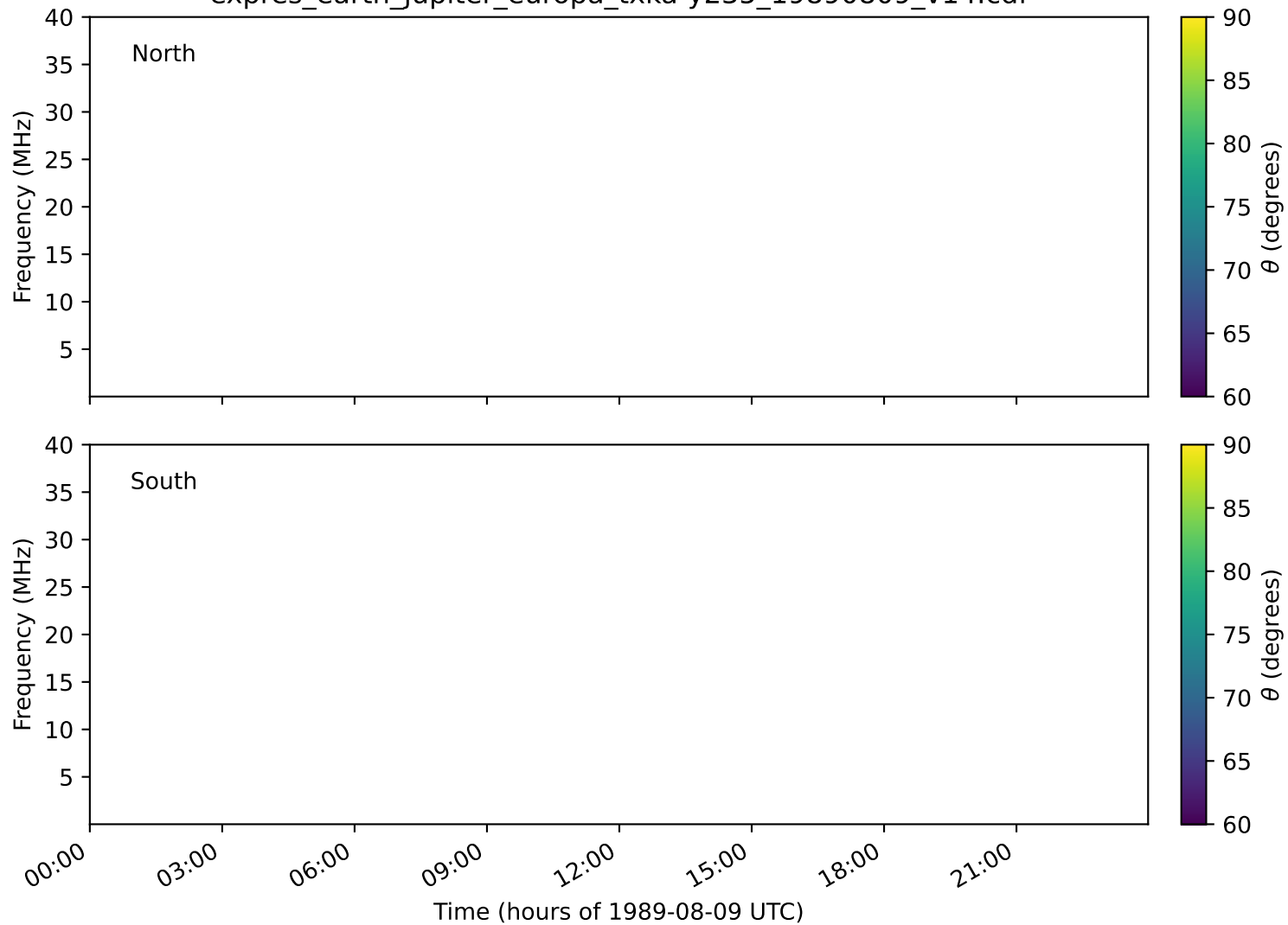
expres_earth_jupiter_europa_txka-y235_19890809_v14.cdf
