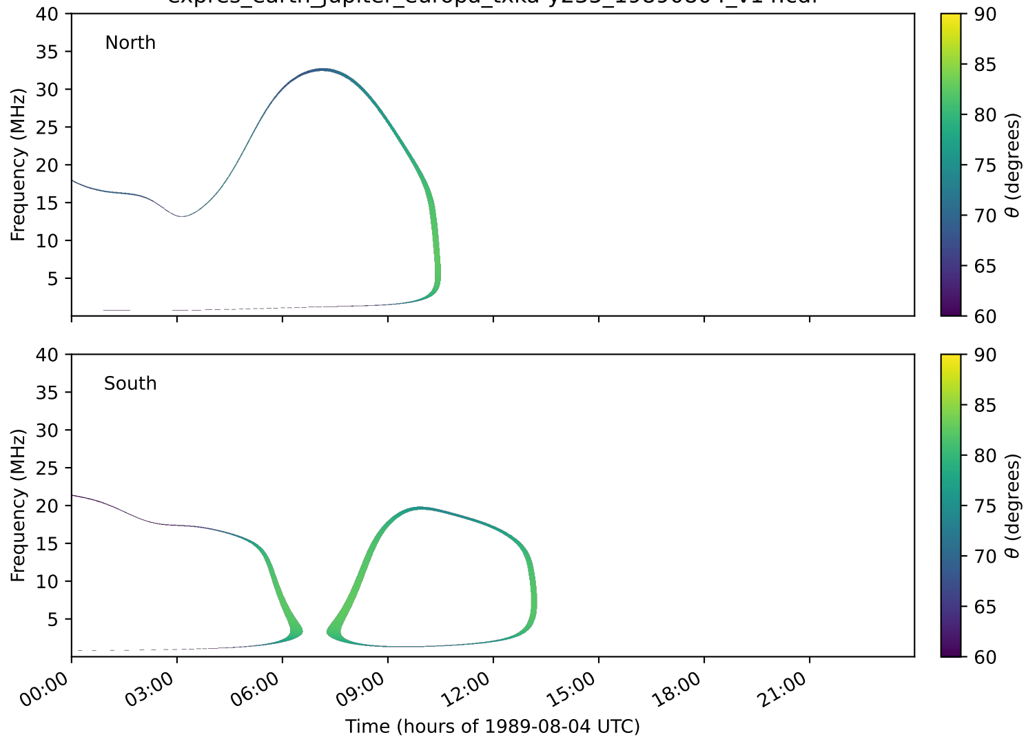
expres_earth_jupiter_europa_txka-y235_19890804_v14.cdf
