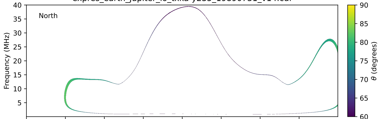
expres_earth_jupiter_io_txka-y235_19890731_v14.cdf
