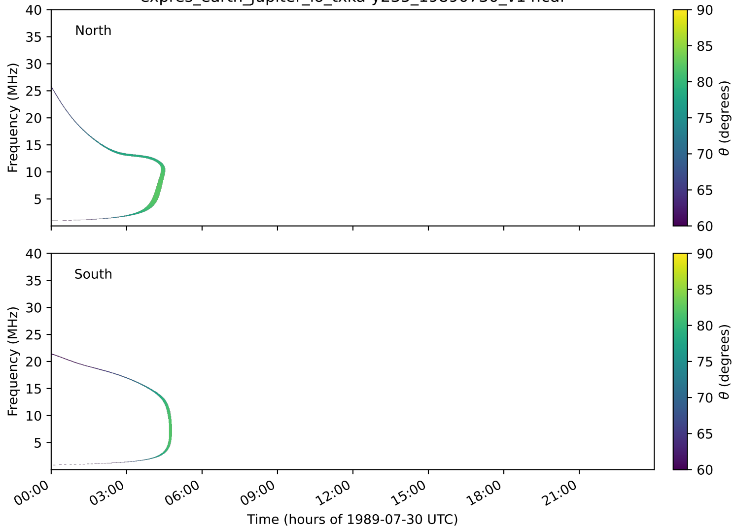
expres_earth_jupiter_io_txka-y235_19890730_v14.cdf
