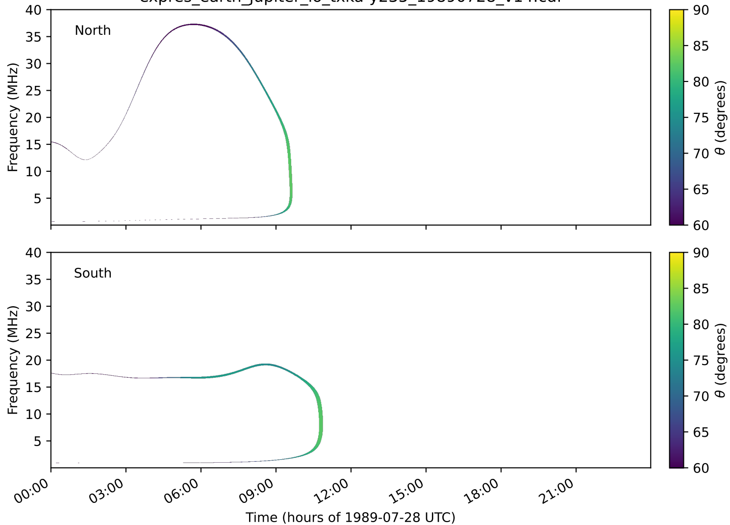
expres_earth_jupiter_io_txka-y235_19890728_v14.cdf
