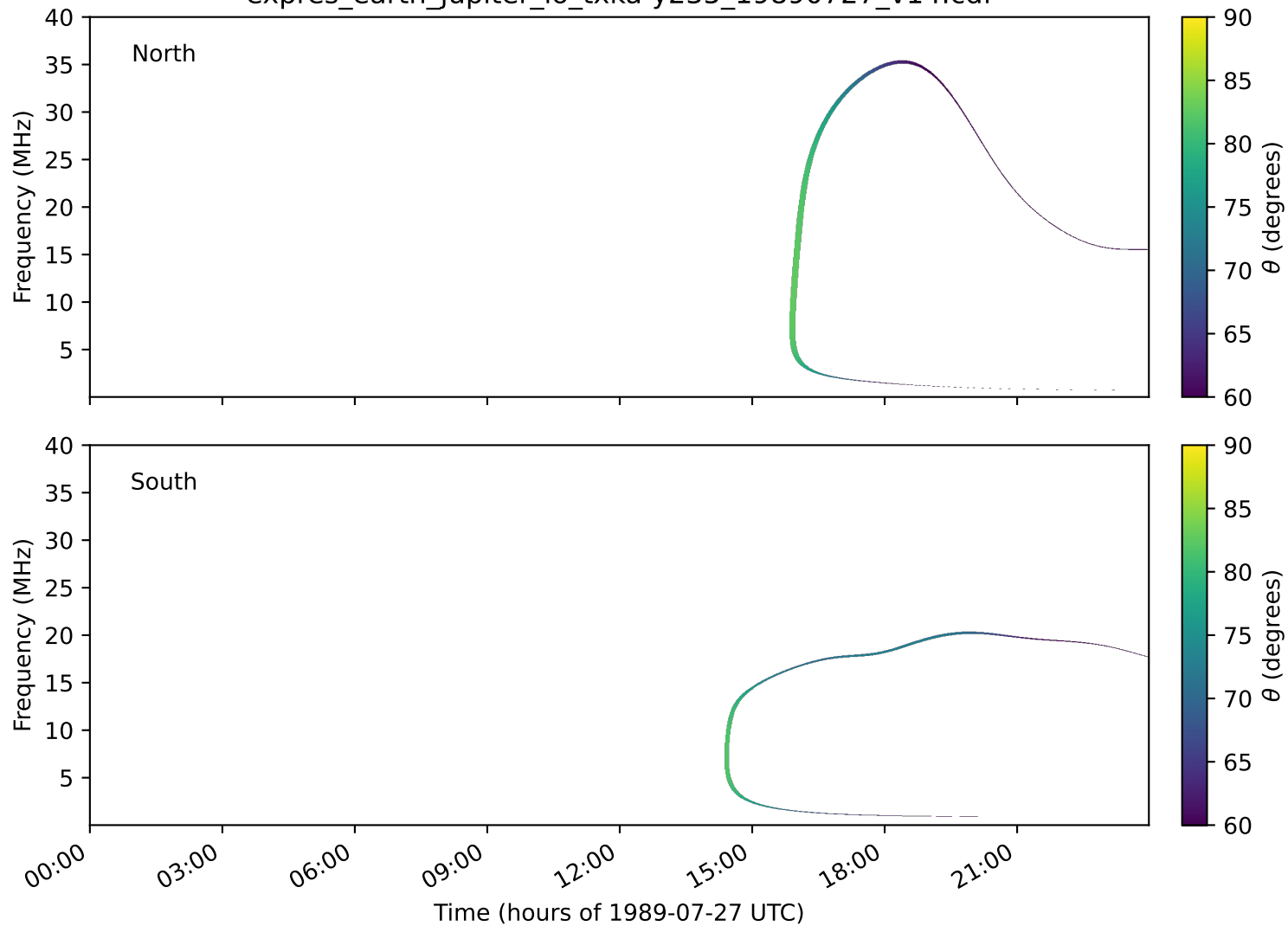
expres_earth_jupiter_io_txka-y235_19890727_v14.cdf
