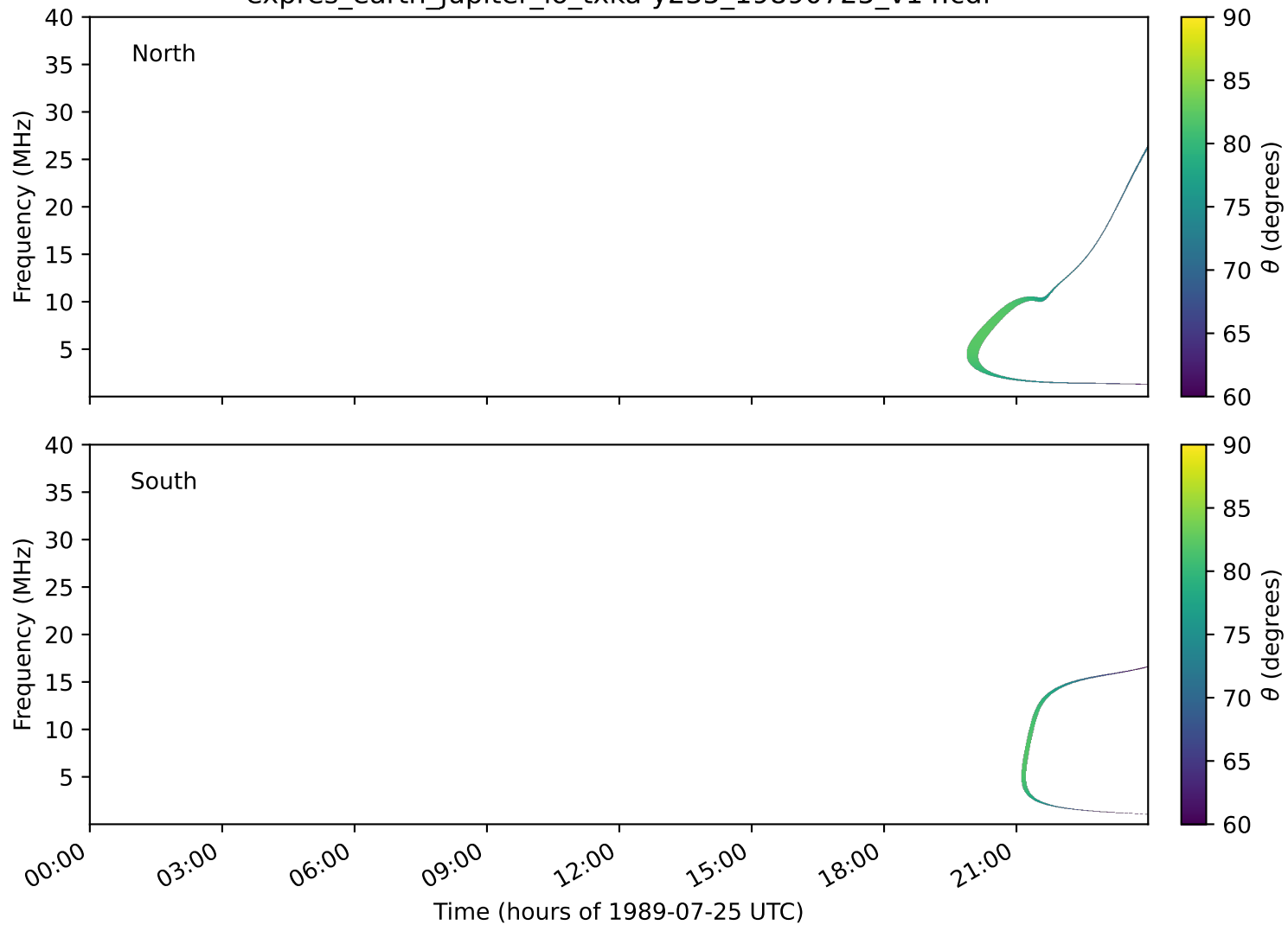
expres_earth_jupiter_io_txka-y235_19890725_v14.cdf
