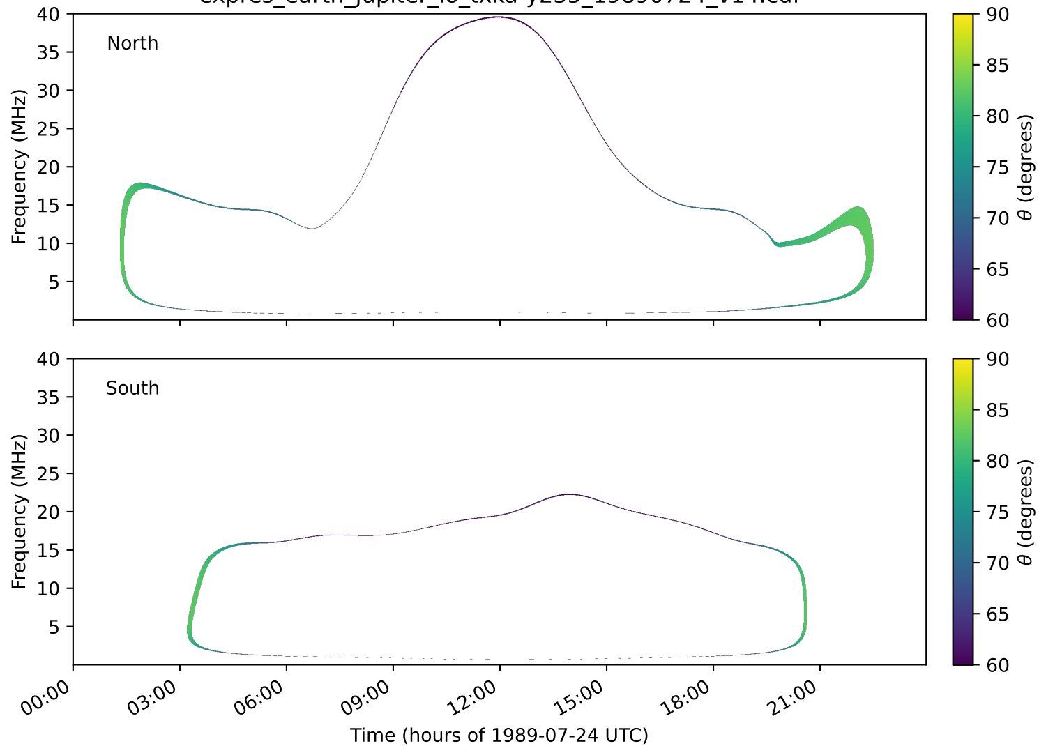
expres_earth_jupiter_io_txka-y235_19890724_v14.cdf
