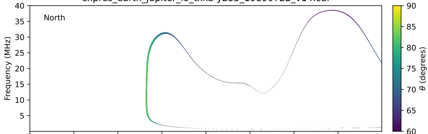
expres_earth_jupiter_io_txka-y235_19890722_v14.cdf
