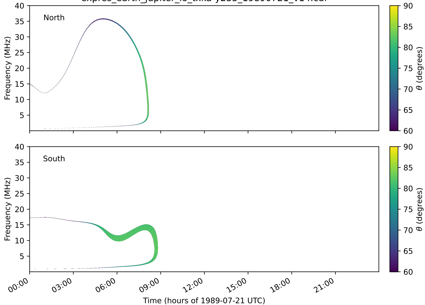
expres_earth_jupiter_io_txka-y235_19890721_v14.cdf
