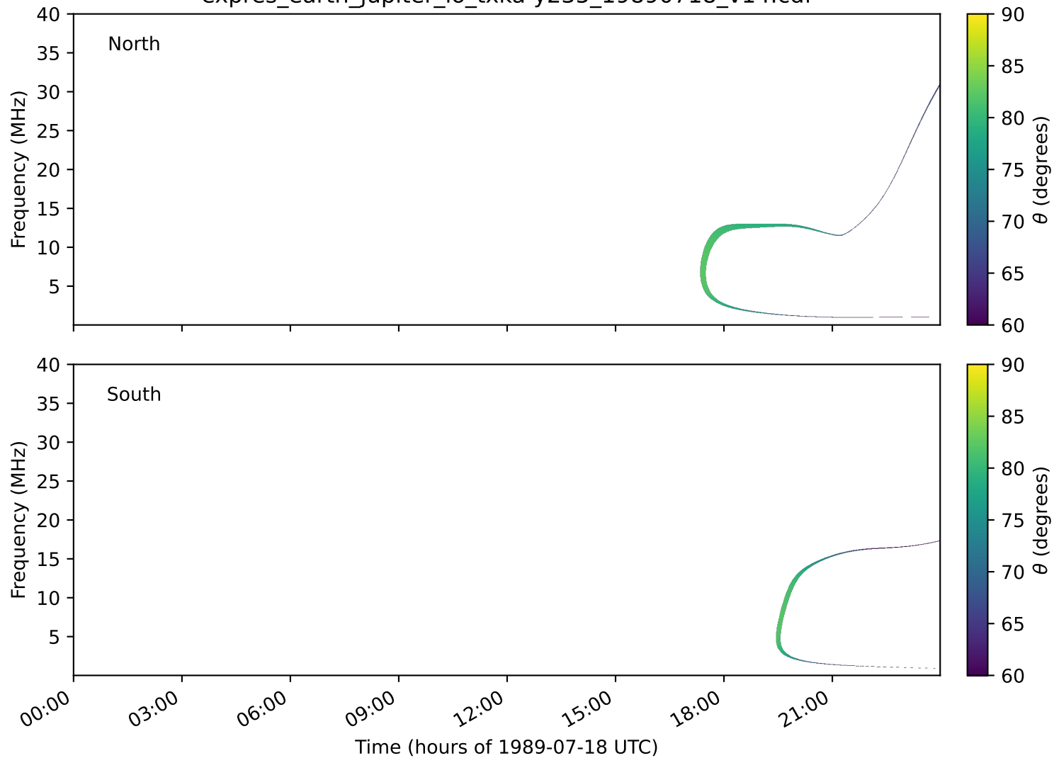
expres_earth_jupiter_io_txka-y235_19890718_v14.cdf
